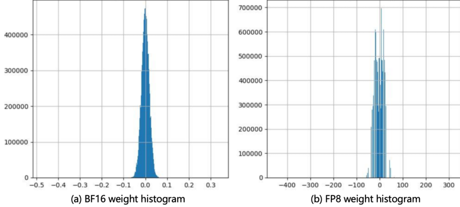
Figure 7: Figure a is the BF16 weight distribution histogram of hunyuan-4b-instruct, and Figure b is the weight distribution histogram after FP8 quantization. It can be seen that the weight distribution after quantization is slightly smoothed to a position far away from 0.
