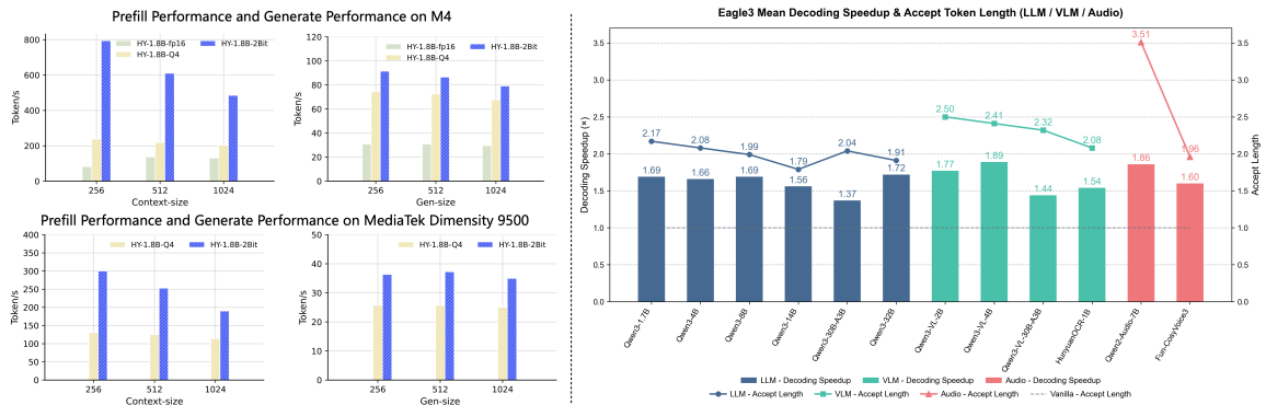
Figure 1: (Left) the edge efficiency of HY-1.8B-2bit. (Right) the speedup of speculative sampling.
