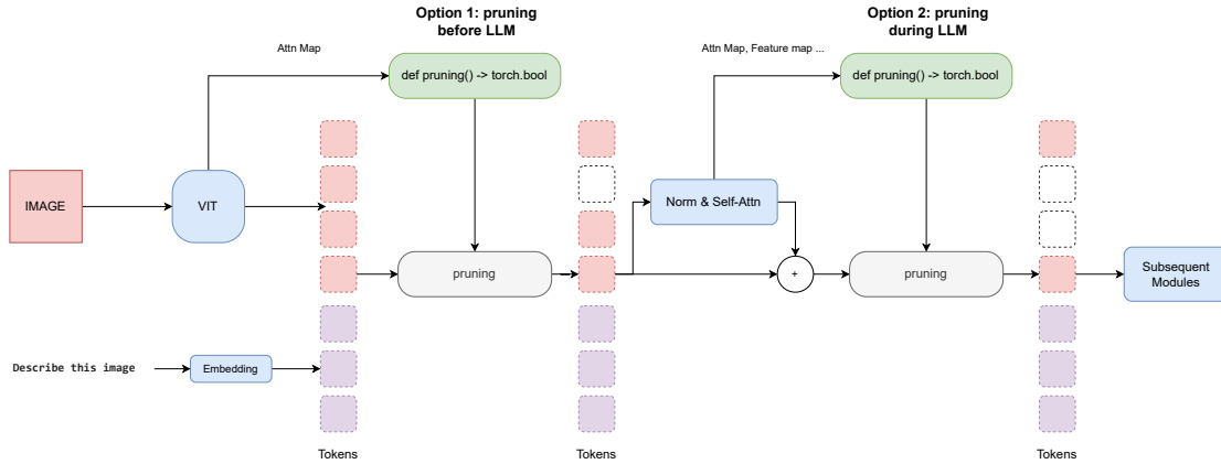
Figure 12: Architecture of the Universal Metadata-Driven Token Pruning Framework. The framework streamlines the pruning process by supporting two flexible compression schedules: Option 1 (Global Pruning) reduces the sequence length before entering the LLM by utilizing metadata from the Vision Tower (e.g., Attention Maps); Option 2 (Layer-wise Pruning) enables incremental sparsification between Transformer blocks based on intermediate states such as feature maps. The core design abstracts the pruning logic into a standardized interface ( def pruning() -> torch.bool ), effectively decoupling the algorithmic strategy from the underlying model architecture.
