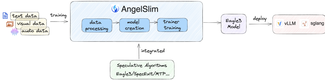
Figure 8: AngelSlim speculative training framework. The framework unifies data processing, model construction, and trainer-level execution to support target-model-dependent draft model training.
