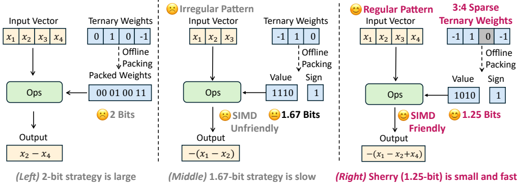
Figure 4: (Left) 2-bit strategy packs each weight into 2 bits to maintain alignment, resulting in large bit wastage. (Middle) 1.67-bit strategy packs 3 weights into 5 bits, introducing SIMD-unfriendly 3-way patterns, leading to slow speed. (Right) Our Sherry enforces a 3:4 sparsity and packs 4 weights into 5 bits, introducing SIMD-friendly 4-way patterns, achieving a small 1.25-bit width and faster inference speed.
