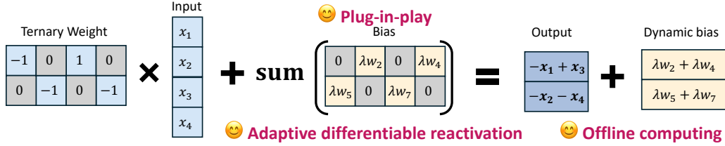
Figure 3: Tequila reactivates dead weights as adaptive dynamic biases via a differentiable function, achieving significant accuracy improvements with nearly zero inference overhead.
