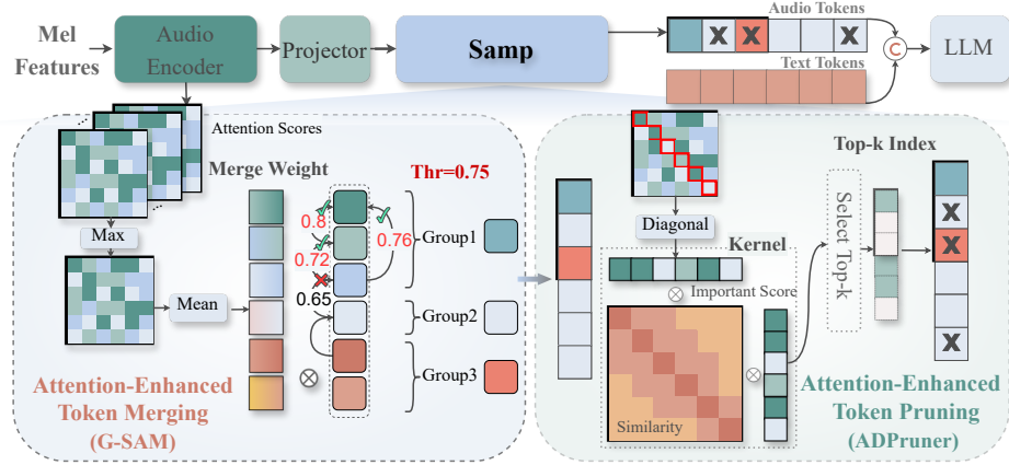
Figure 14: Architecture of the proposed Samp with adaptive merge-prune fusion. By introducing a similarity threshold, Samp dynamically balances token merging and pruning, according to speech temporal structures. Similar tokens are first adaptively merged to maximize information retention, followed by pruning to reduce redundancy and improve diversity under high compression rates.
