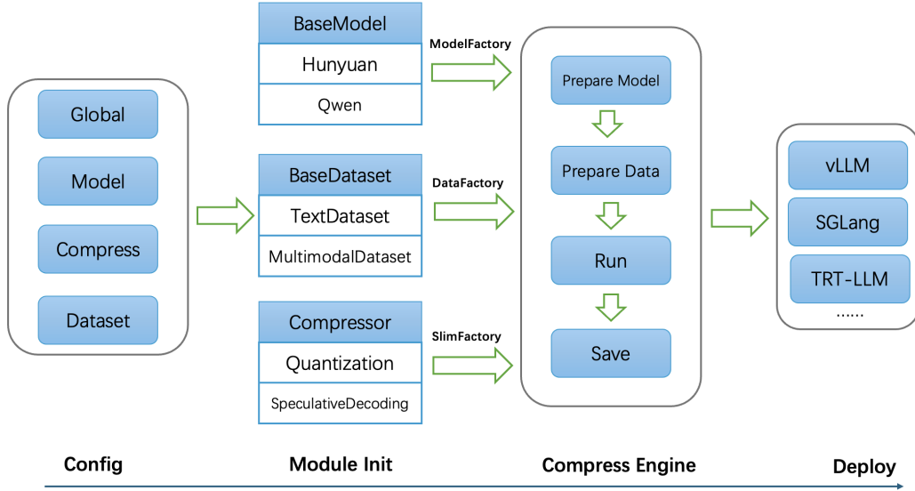
Figure 6: AngelSlim Quantization Framework.
