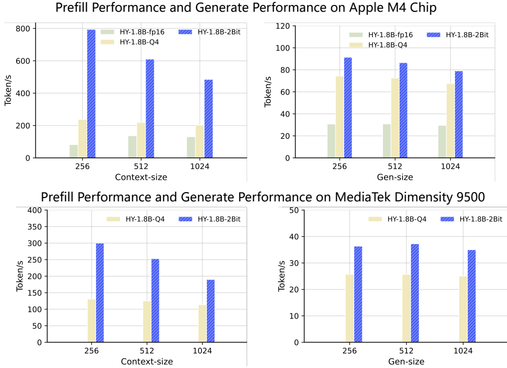
Figure 2: Comparison of inference latency (TTFT) and generation throughput on edge devices. HY-1.8B-2Bit consistently outperforms both 4-bit and FP16 baselines across varying sequence lengths.
