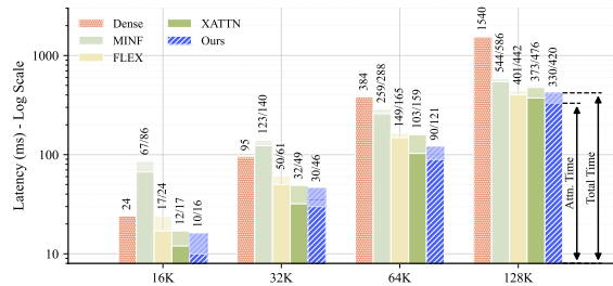
Figure 11: Latency comparison (ms) on Nvidia GPU. Results are reported as Attention Kernel Time/Total Time.
