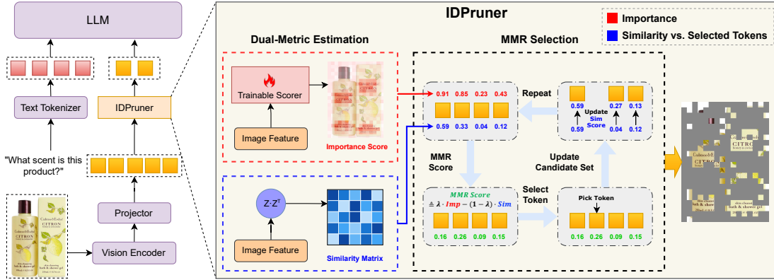
Figure 13: Architecture of the proposed IDPruner with importance-diversity optimization. By computing Importance Scores and a Similarity Matrix, IDPruner dynamically balances token saliency and semantic diversity through an MMR-based iterative selection process.
