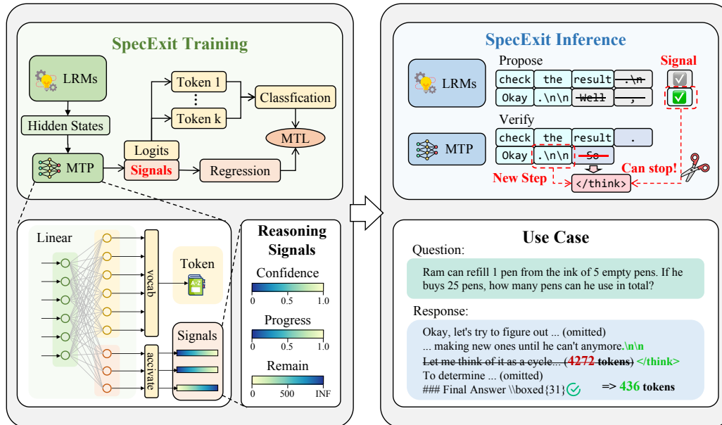
Figure 9: Overall architecture of the proposed SpecExit framework. The Multi-Token Prediction (MTP) layer is augmented to output both token logits and auxiliary signals. Training is performed with multi-task learning, while at inference these signals guide speculative early stopping without modifying the backbone model. The example illustrates how redundant reasoning steps can be pruned while preserving final answer quality.
