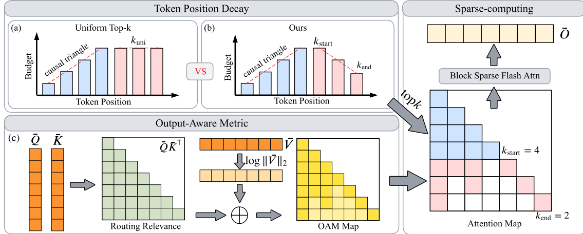
Figure 10: Architecture of the proposed Stem. (a) Uniform Sparse Attention: Illustrates the traditional method applying a fixed top-k budget across all token positions, often leading to information loss in initial tokens. (b) Token Position-Decay (TPD): Contrasts with (a) by allocating dynamic budgets, assigning higher retention stability to initial tokens ("recursive anchors") to preserve causal structure. (c) Output-Aware Metric (OAM): A selection metric combining attention scores with value vector magnitudes to minimize output approximation error.
